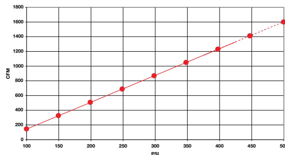
Super Dominator 600 Air Consumption
