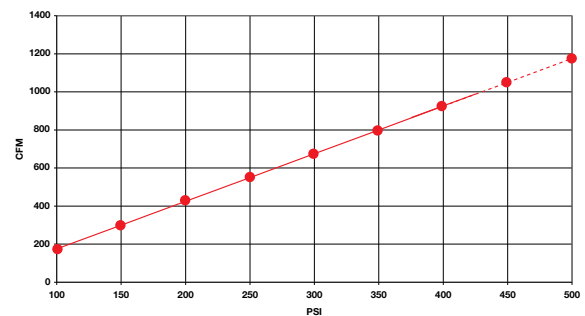
Super Dominator 500 Air Consumption
