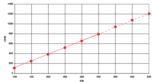
Mach 50 Air Consumption
