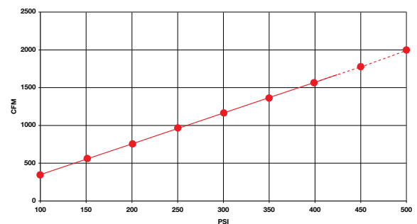
Dominator 750 Air Consumption
