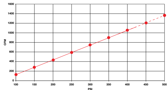
Mach 60 Air Consumption
