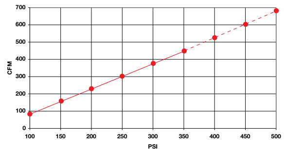
Dominator 350 Air Consumption
